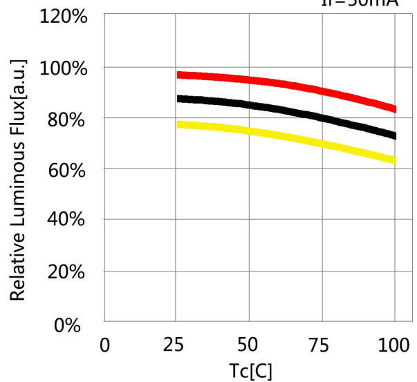
Temperature vs. Relative Luminous Flux If=50mA
